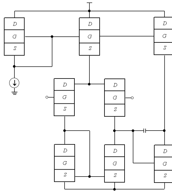
Fig1a. Structure of the considered amplifier [19]
