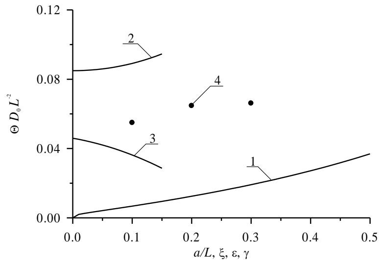
Fig7. Dependences of dimensionless optimal annealing time for doping by ion implantation, which have been obtained by minimization of mean-squared error, on several parameters. Curve 1 is the dependence of dimensionless optimal annealing time on the relation a/L and \xi = \gamma = 0 for equal to each other values of dopant diffusion coefficient in all parts of heterostructure. Curve 2 is the dependence of dimensionless optimal annealing time on value of parameter \epsilon for a/L=1/2 and \xi = \gamma = 0 . Curve 3 is the dependence of dimensionless optimal annealing time on value of parameter \xi for a/L=1/2 and \epsilon = \gamma = 0 . Curve 4 is the dependence of dimensionless optimal annealing time on value of parameter \gamma for a/L=1/2 and \epsilon = \xi = 0
