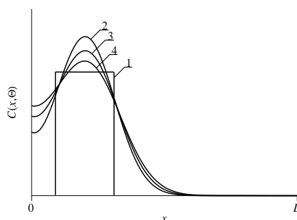
Fig4a. Distributions of concentration of infused dopant in depth of heterostructure from Fig. 1 for different values of annealing time (curves 2-4) and idealized step-wise approximation (curve 1). Increasing of number of curve corresponds to increasing of annealing time
