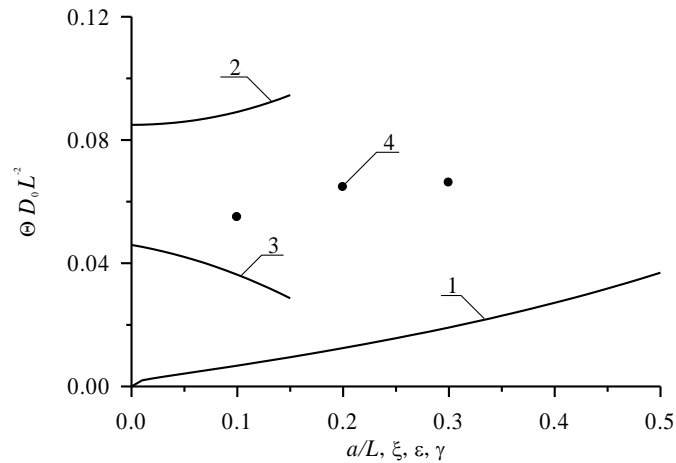
Fig5b. Dimensionless optimal annealing time of implanted dopant as a function of several parameters. Curve 1 describes the dependence of the annealing time on the relation a/L and \xi=\gamma=0 for equal to each other values of dopant diffusion coefficient in all parts of heterostructure. Curve 2 describes the dependence of the annealing time on value of parameter \epsilon for a/L=1/2 and \xi=\gamma=0 . Curve 3 describes the dependence of the annealing time on value of parameter \xi for a/L=1/2 and \epsilon=\gamma=0 . Curve 4 describes the dependence of the annealing time on value of parameter \gamma for a/L=1/2 and \epsilon=\xi=0
